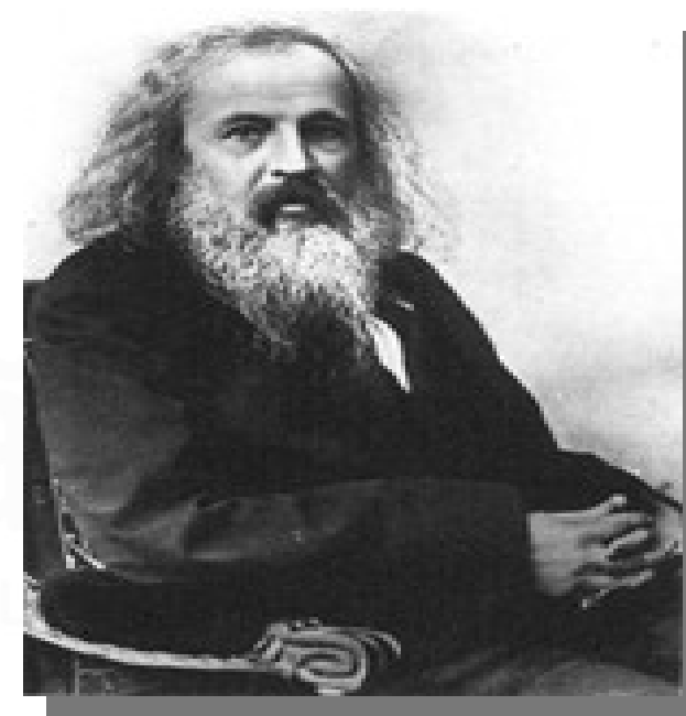
Mendeleiev
